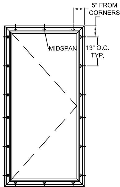
TYPICAL ELEVATION WITH FASTENER SPACING
